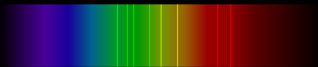
A_7
