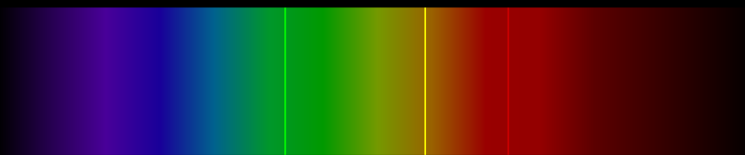
Petersen Graph
